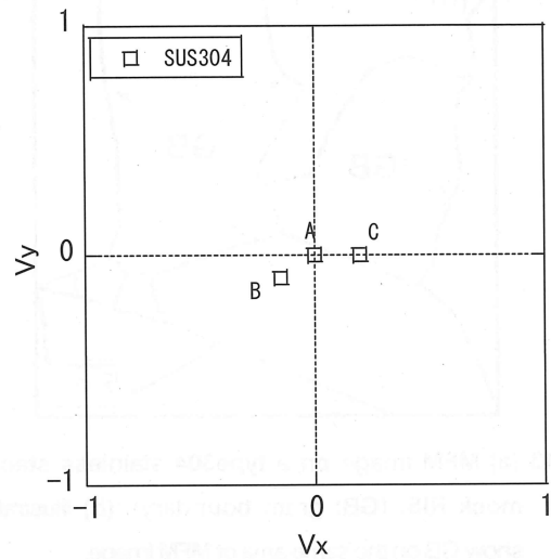
Fig.11 Probe voltage distribution on phase plane obtained by Eddy current measurement on type304 stainless steels with mock RIS.
