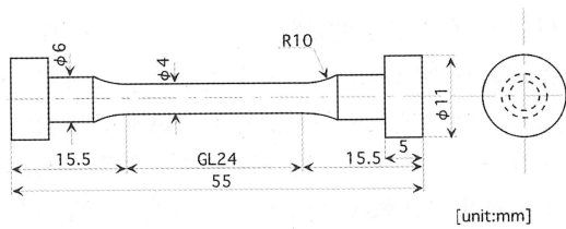
Fig.1 The specimen for SSRT test (1) [3-6]
