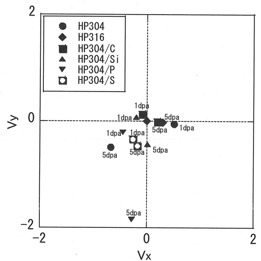
Fig.5 Probe voltage distribution on phase plane obtained by Eddy current measurement on neutron irradiated high purity stainless steels.
