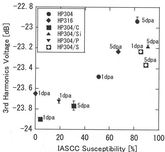
Fig.4 Correlation between IASCC susceptibility and 3rd harmonics voltage on neutron irradiated high purity stainless steels [3-6] .
