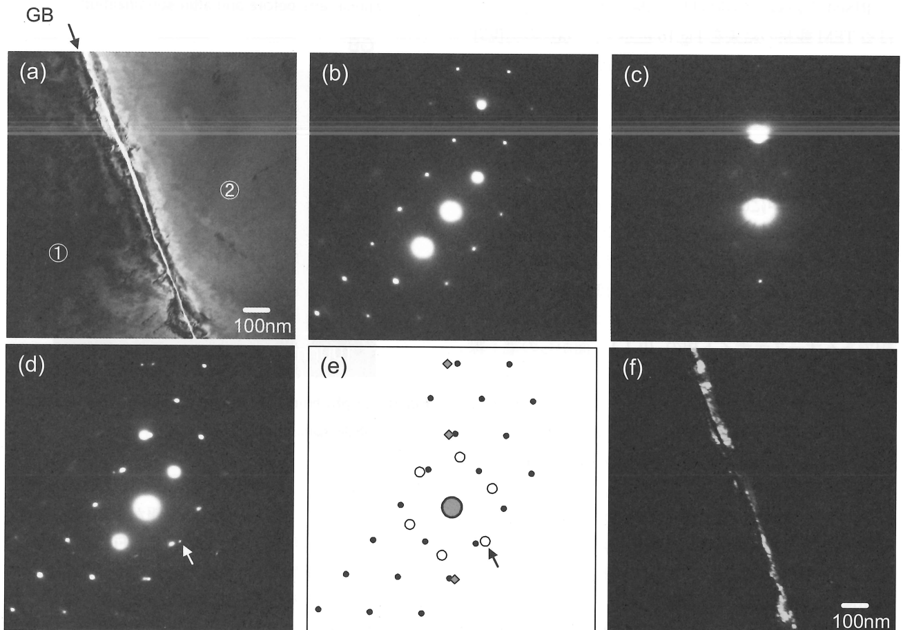
Fig.16 TEM observation results on thermally sensitized RIS04, including grain boundary (GB) region. (a) Bright field image, (b) Diffraction pattern from the grain①( B=[0\ 1\ 1] ), (c) Diffraction pattern from the grain② ( B=[1\ 3\ 3] ), (d) Diffraction pattern from the region including grain①, ② and GB. (e) An illustration of (d) ( \cdot : diffraction spots from grain①, \blacklozenge : grain②, \circ : precipitates along GB (FeNi 3 , B=[0\ 1\ 1] ), (f) Dark field image obtained from the diffraction spot indicated by an arrow in (d) & (e).
