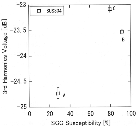
Fig.10 Correlation between SCC susceptibility and 3rd harmonics voltage on type304 stainless steel with mock radiation induced segregation (RIS).
