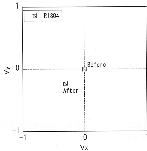
Fig.14 Probe voltage distribution on phase plane obtained by Eddy current measurement on RIS04 specimens before and after sensitization.
