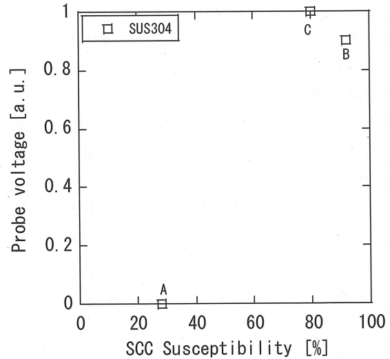
Fig.12 Correlation between SCC susceptibility and probe voltage obtained on type304 stainless steels with mock RIS.
