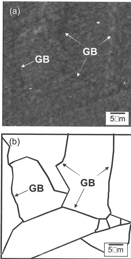
Fig.13 (a) MFM image on a type304 stainless steel with mock RIS. (GB: grain boundary). (b) Illustration to show GB on the same area of MFM image.
