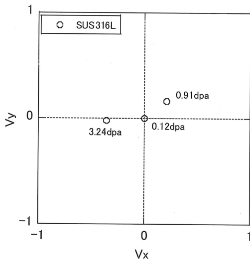
Fig.8 Probe voltage distribution on phase plane obtained by Eddy current measurement on neutron irradiated type316L stainless steels.
