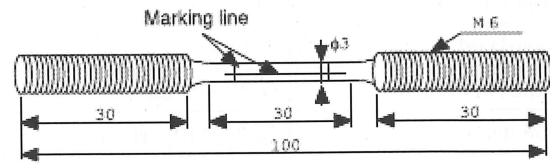
Fig.2 The specimen for SSRT test (2) [9-10]
