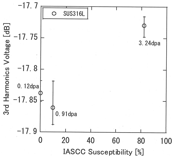
Fig.7 Correlation between IASCC susceptibility and 3rd harmonics voltage on neutron irradiated type316L stainless steels [10].
