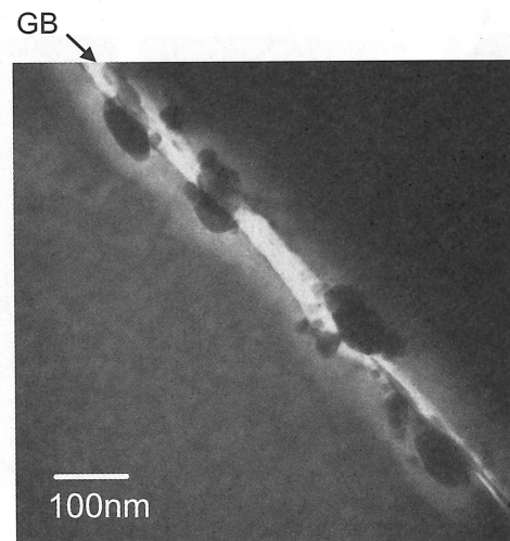
Fig.15 Bright field TEM image on a thermally sensitized RIS04 specimen.
