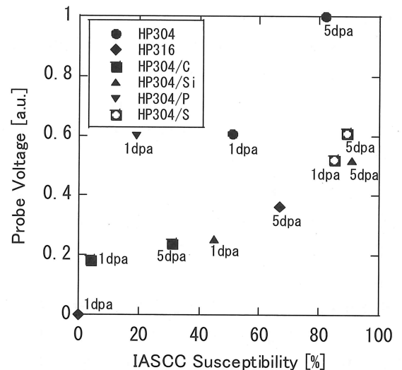
Fig.6 Correlation between IASCC susceptibility and probe voltage obtained on neutron irradiated high purity stainless steels [3-6] .
