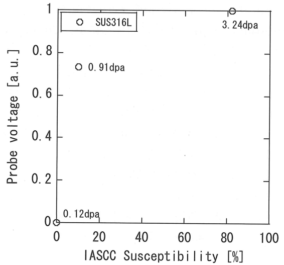
Fig.9 Correlation between IASCC susceptibility and probe voltage obtained on neutron irradiated type316L stainless steels [10].
