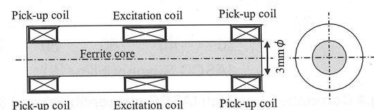
Fig.3 The sensor probe for Eddy current method and AC magnetization method.
