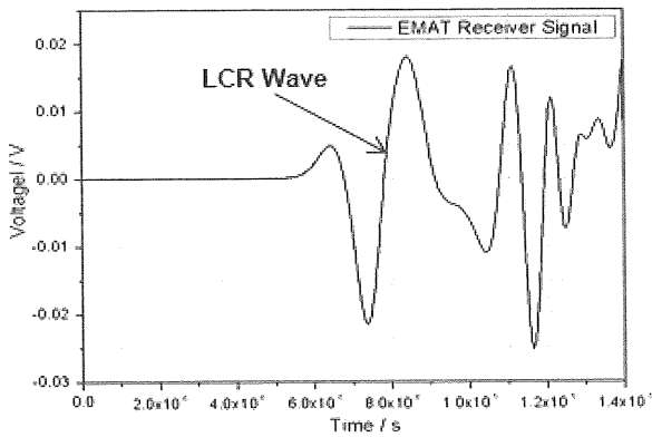
Fig. 4 LCR wave received by EMAT
