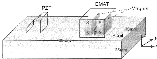
Fig. 2 A pitch-catch setup model in simulation
