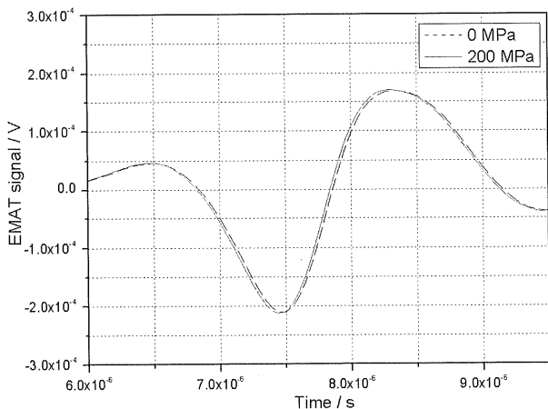
Fig. 6 Acoustoelastic effect in rail steel
