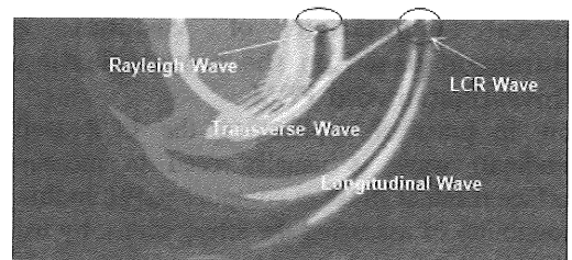
Fig. 3 Ultrasonic wave field excited by PZT
