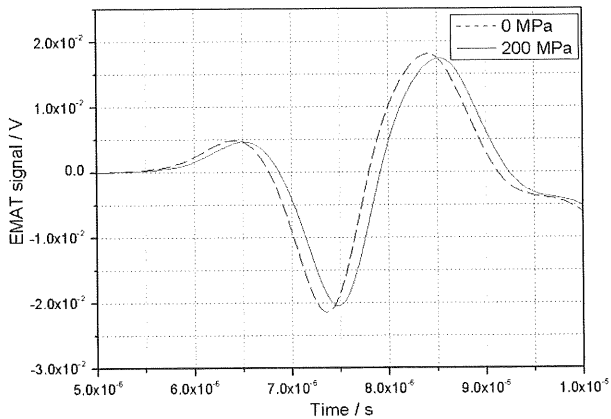
Fig. 5 Acoustoelastic effect in Al alloy
