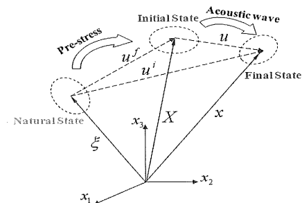
Fig. 1 Coordinates for material point in three states
