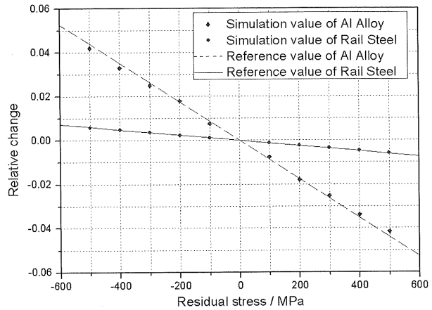
Fig.7 Relative change of LCR wave's speed in Al Alloy and rail steel
