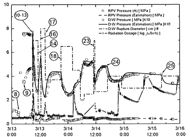
Fig. 6 Transient pressure, radiation dosage and estimated rupture area of D/W
