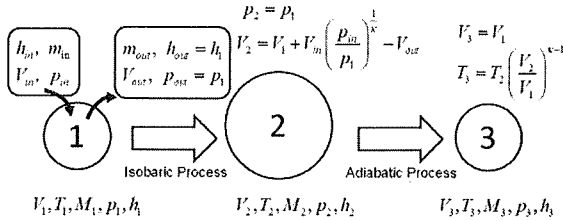
Fig. 4 Thermodynamic model of pressure vessel
