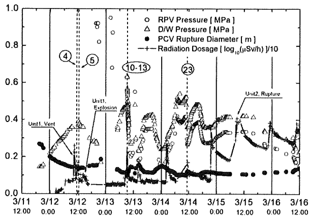
Fig. 2 Plant parameters, radiation dosage and estimated rupture diameter of PCV
