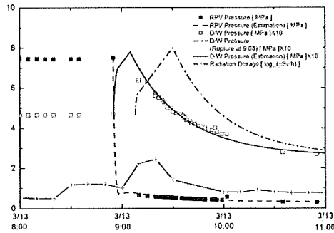
Fig. 5 Transient pressure, radiation dosage and estimated rupture area of D/W, just after the breakage
