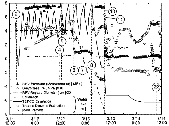
Fig. 1 Plant parameters, estimated water levels and rupture diameter of RPV
