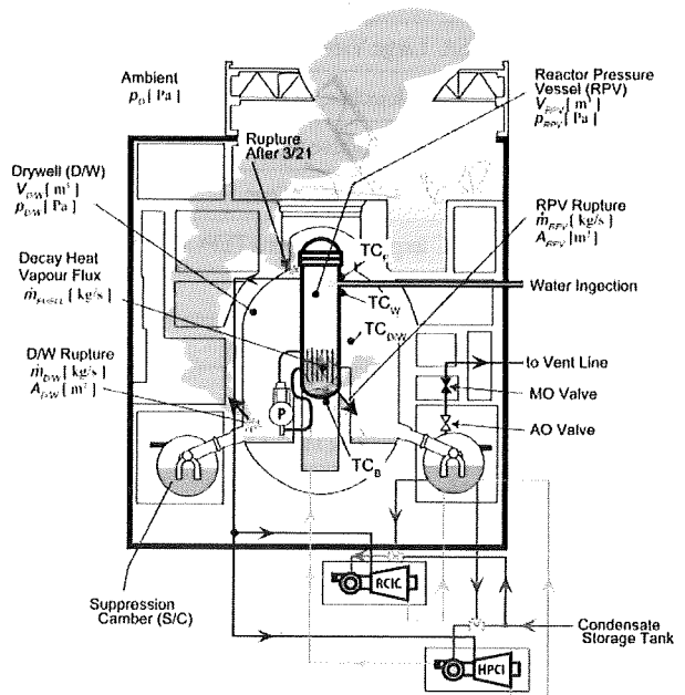
Fig. 3 Physical model of Unit 3
